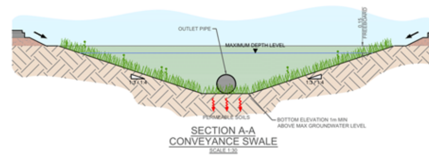
FIGURE D3 SCHEMATIC LAYOUT SHOWING TYPICAL FEATURES OF SWALES
